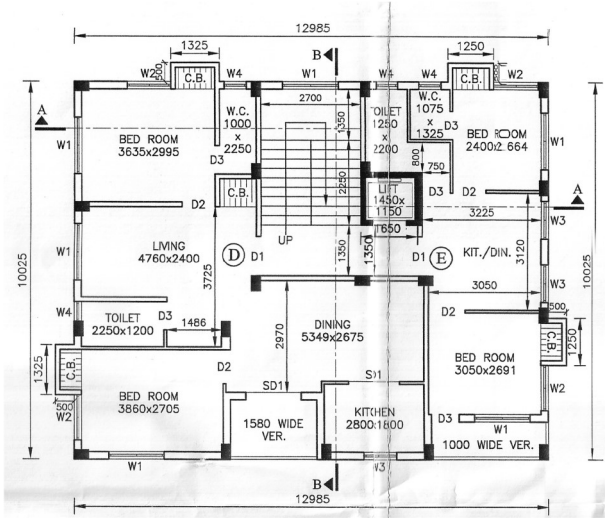
TYPICAL FLOOR PLAN (2ND & 4TH FLOOR PLAN)
